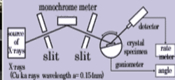
3. Angle measurement
